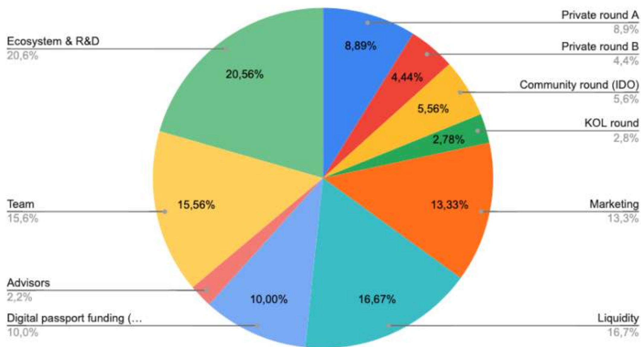
Token distribution
